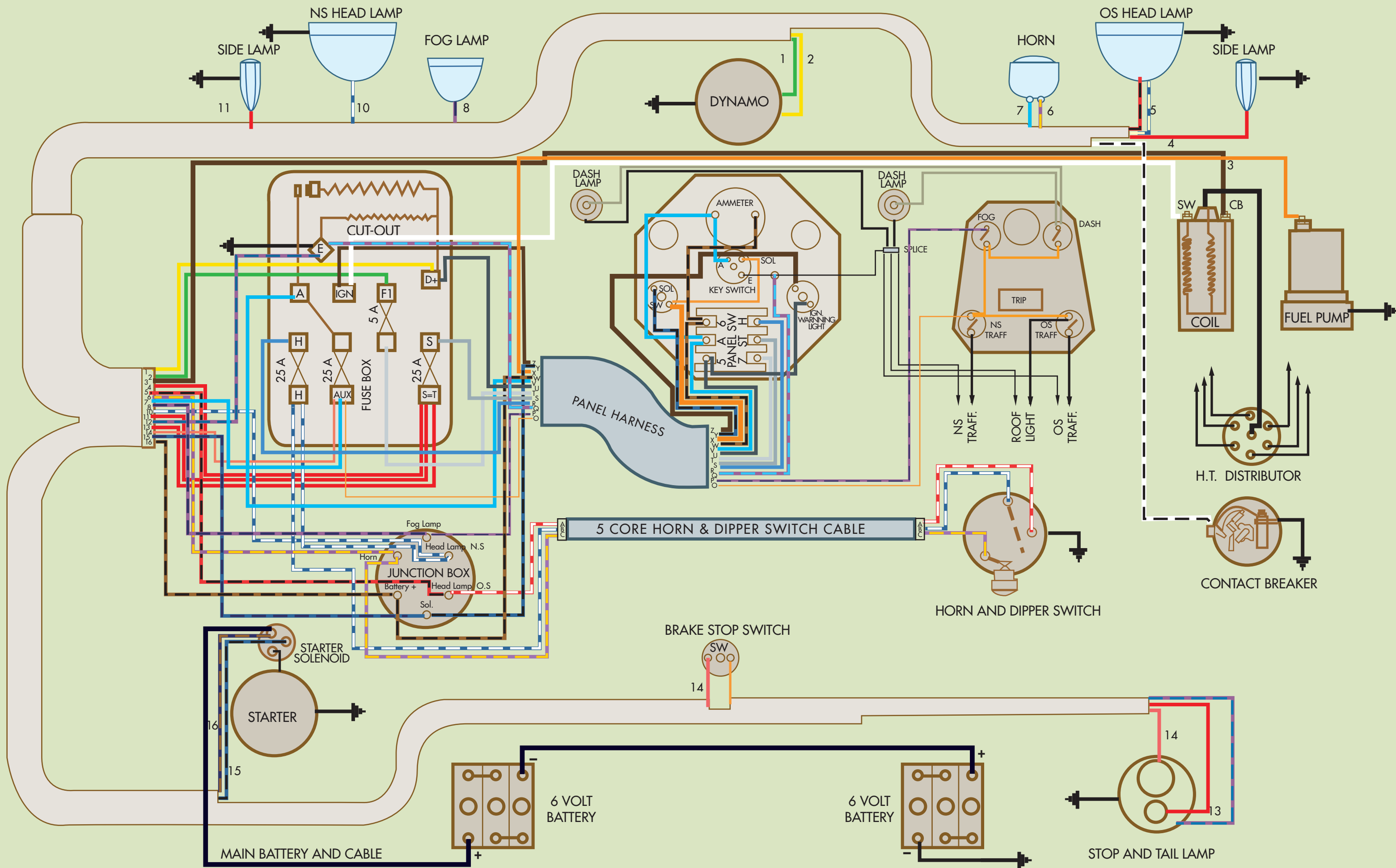
WIRING DIAGRAM FOR THE MAGNETTE "KN" TYPE
